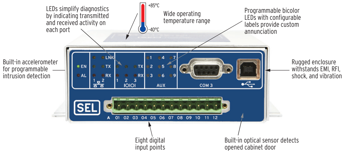
Figure 5 SEL-3505-3 Front-Panel View
